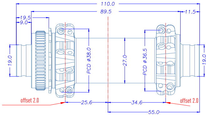
Front Hub
