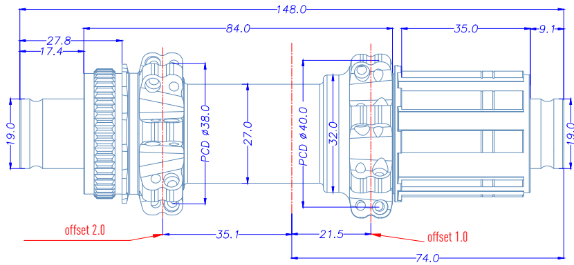
Rear Hub
